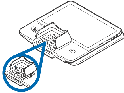
Figure 14 Installing the Privacy Shield
