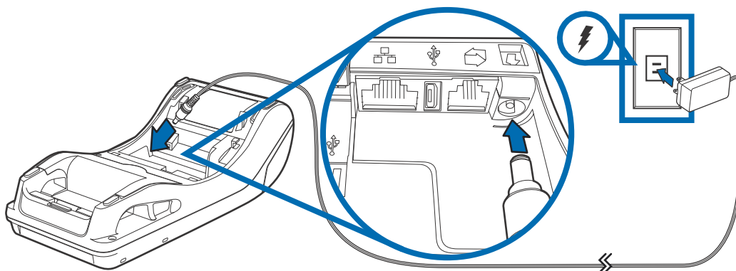
Figure 16 Connecting the Power Pack
