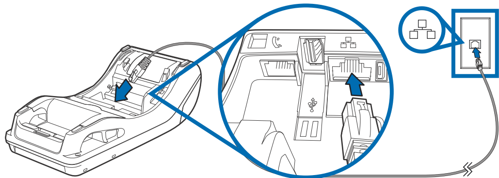
Figure 11 Ethernet Connection
