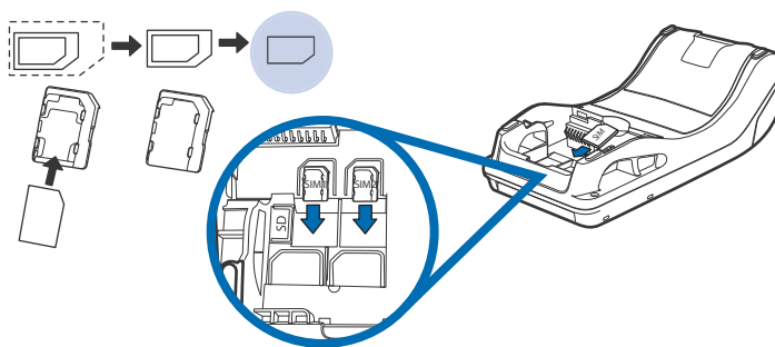
Figure 9 Inserting the Nano SIM in Micro SIM Adaptor
