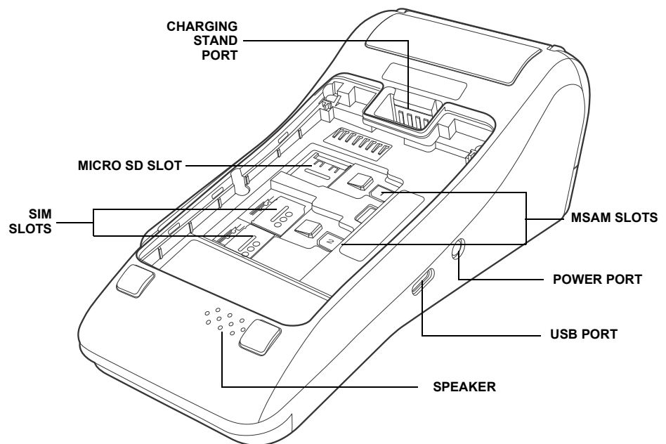
Figure 2 V400m Underside
